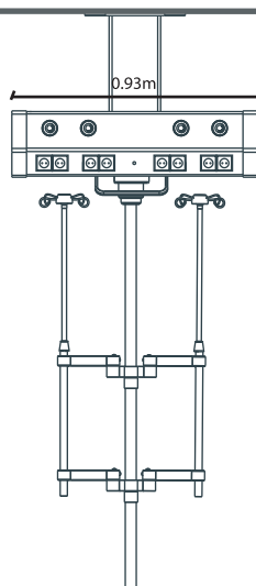
SLIDING IV DROPPER
