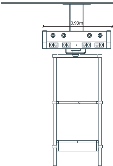
SLIDING SHELF AND DRAWER T.P-SH-D-R
